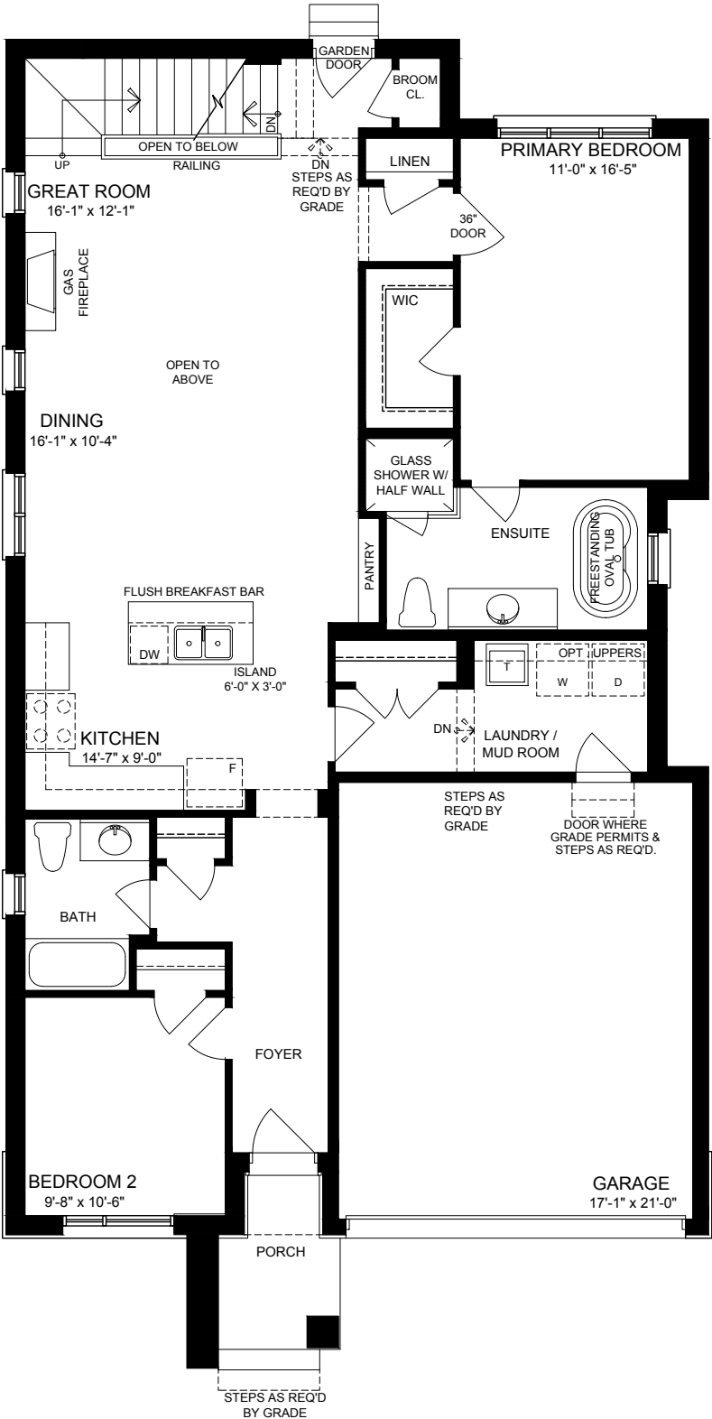
MAIN FLOOR W/ OPTIONAL LOFT
